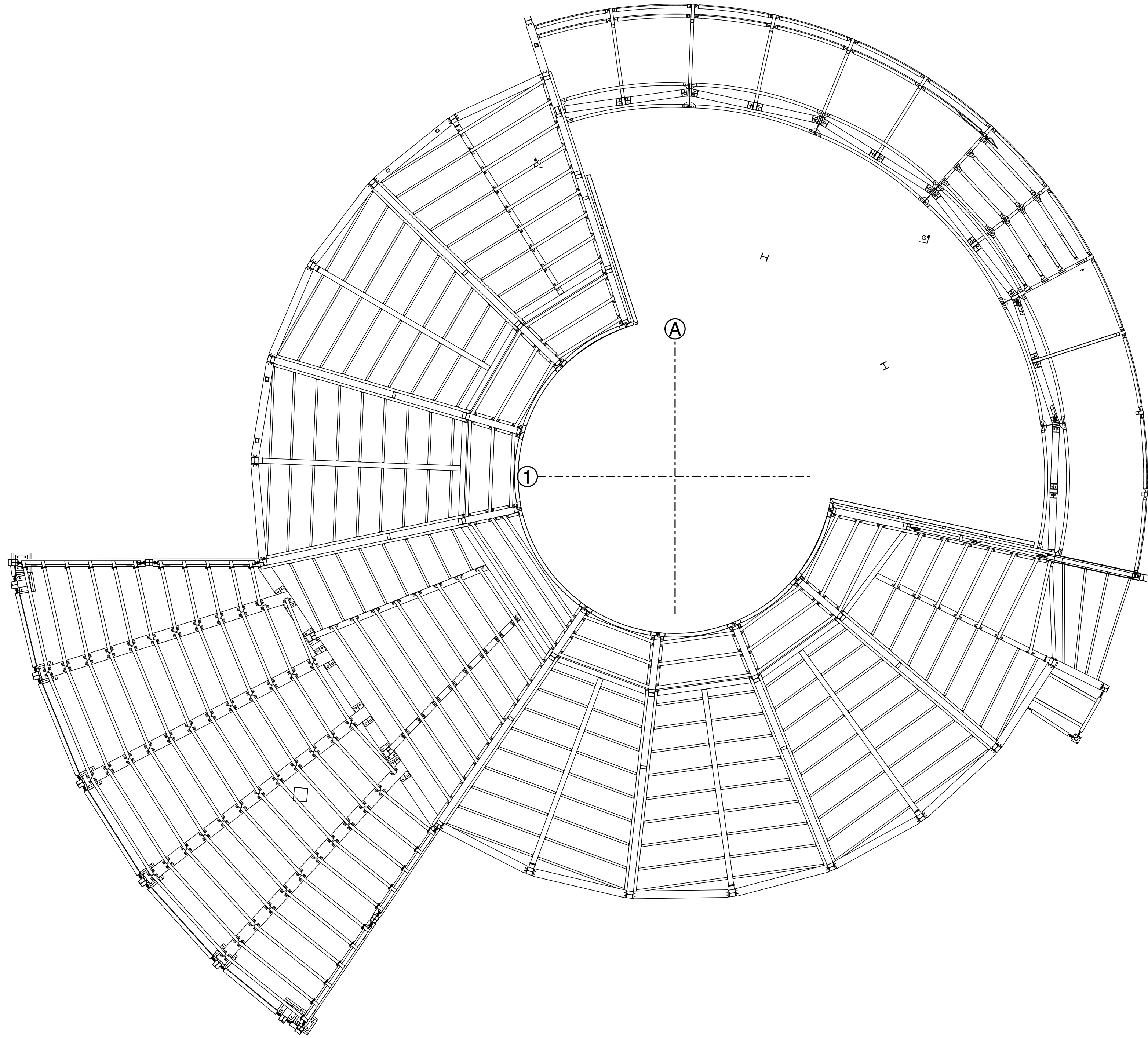
View 01 (3d)
