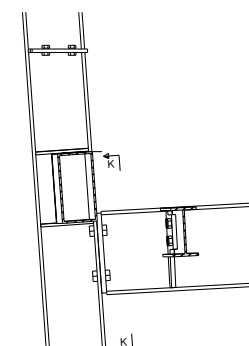
DETAIL D
