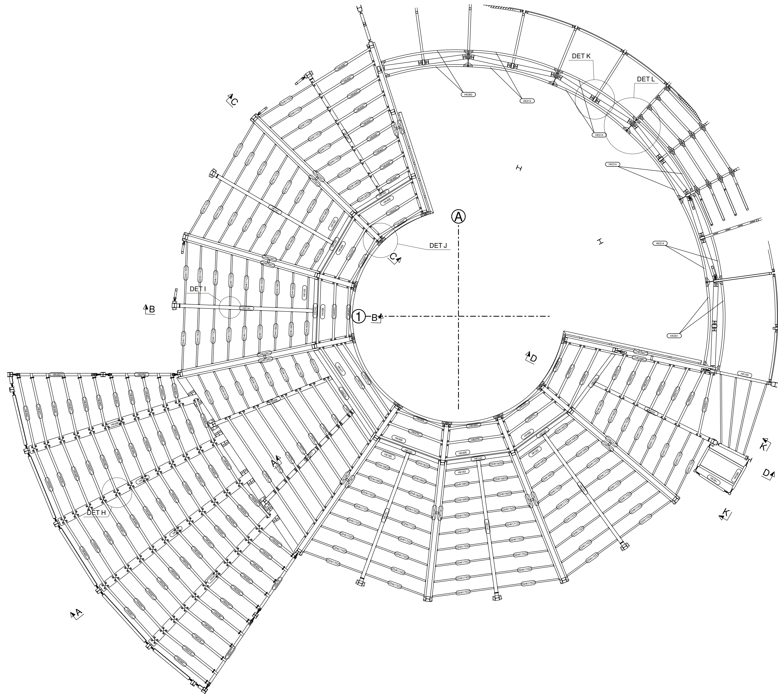
PLAN +4.00
