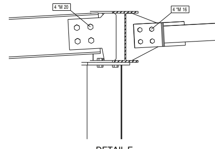
DETAIL E
