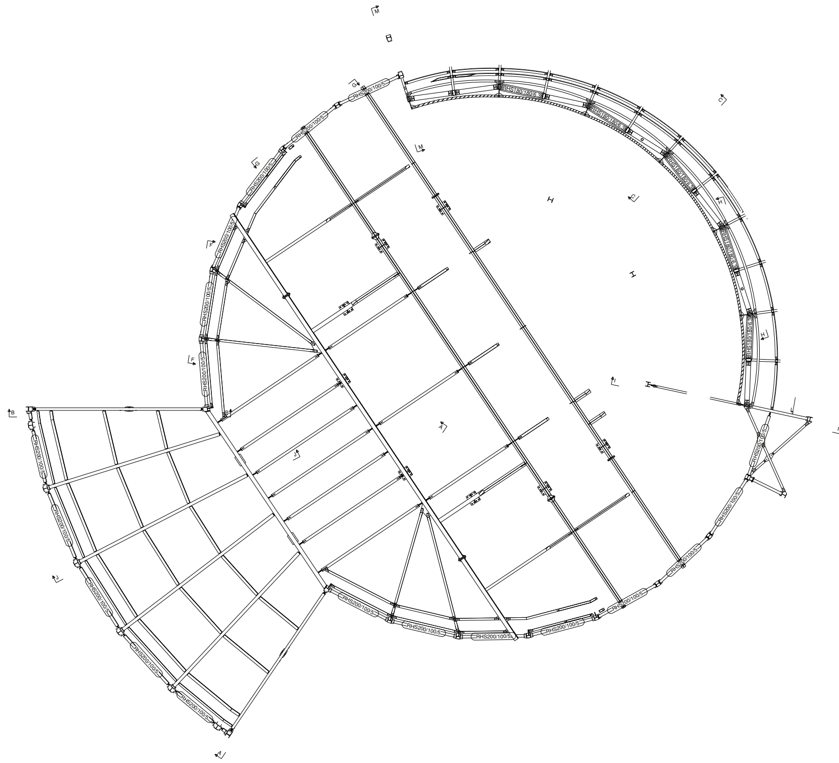
View_02 (3d)
