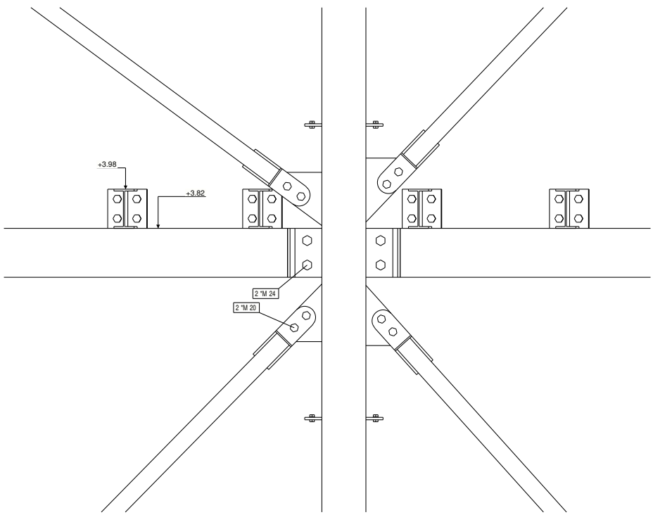
DETAIL A
