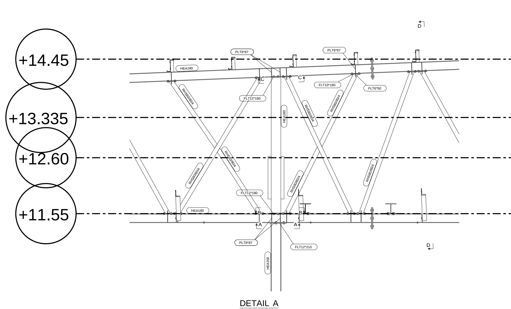
DETAIL A
