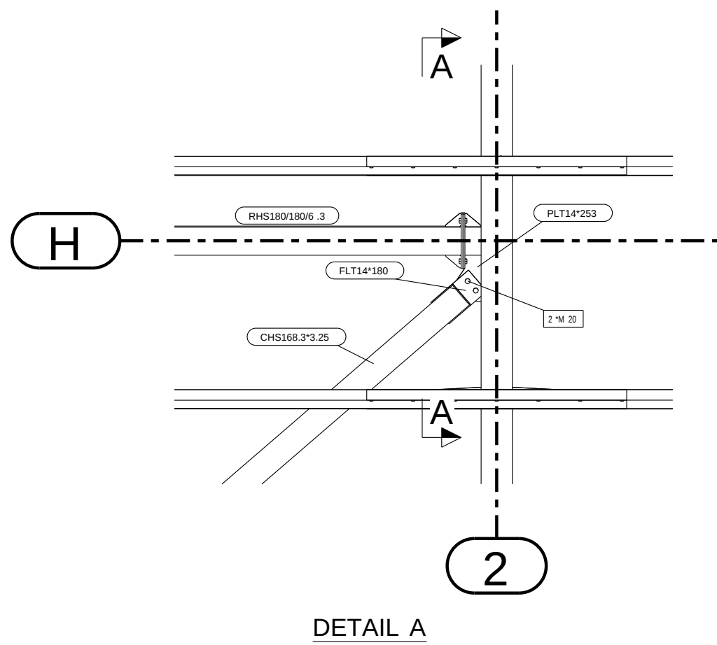
DETAIL A
