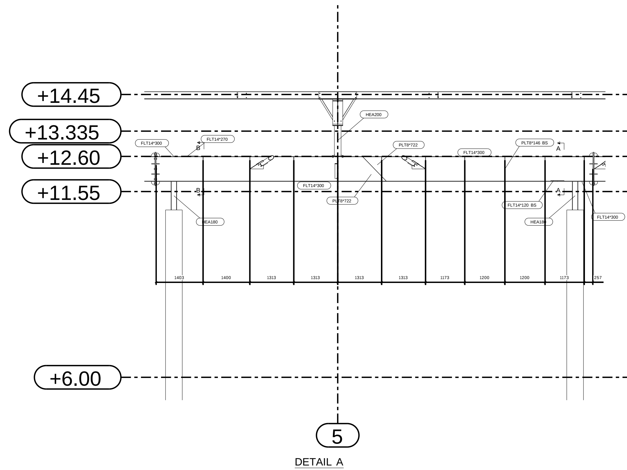
DETAIL A
