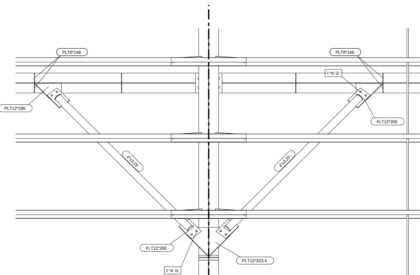
DETAIL B
