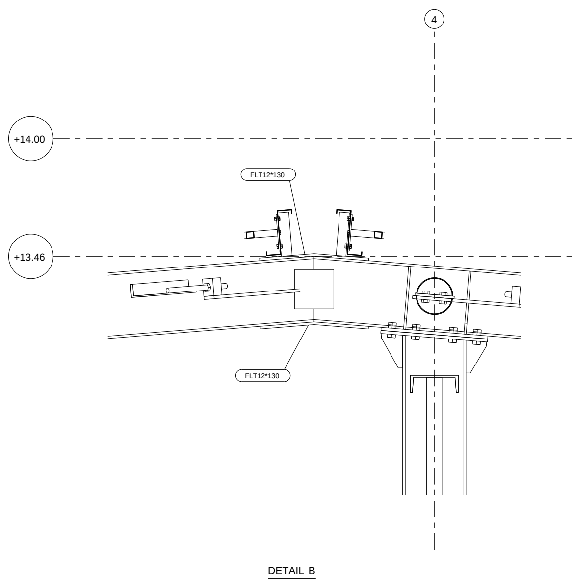
DETAIL B
