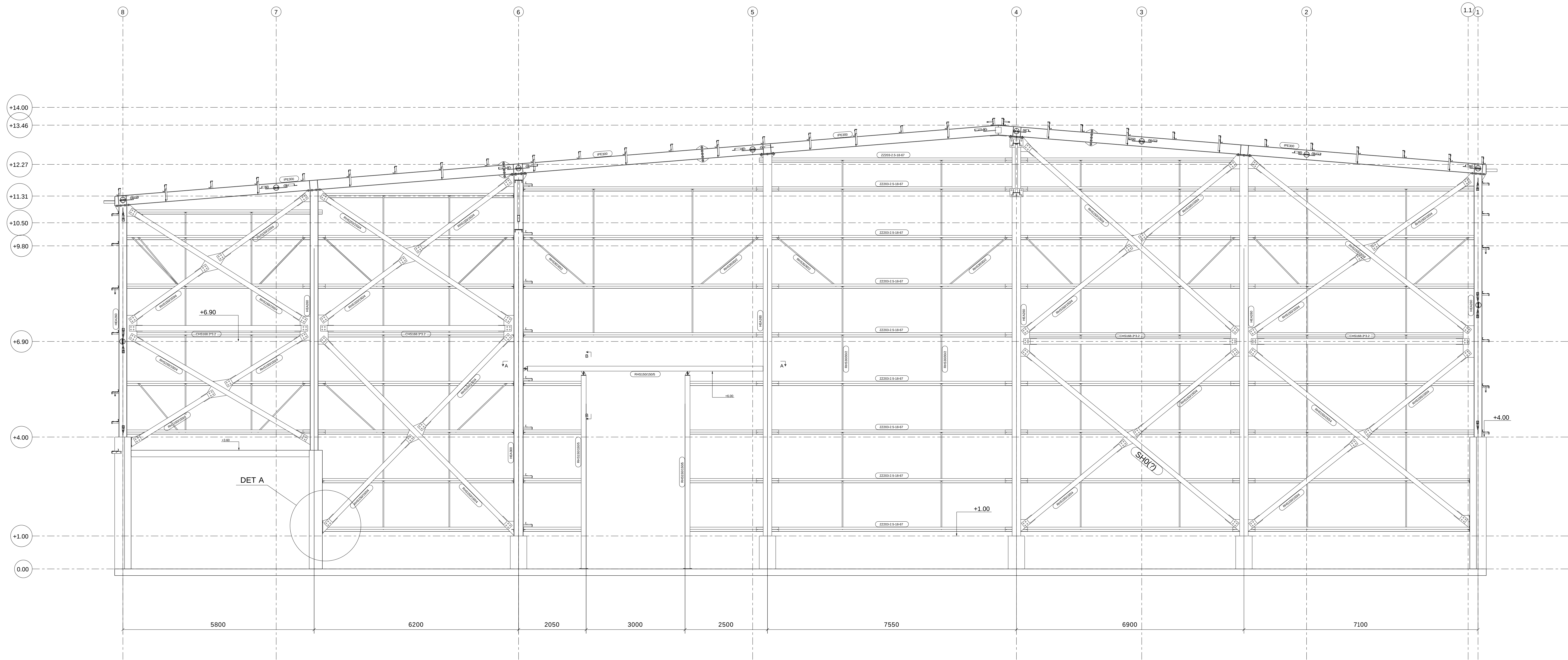
Grid Q
