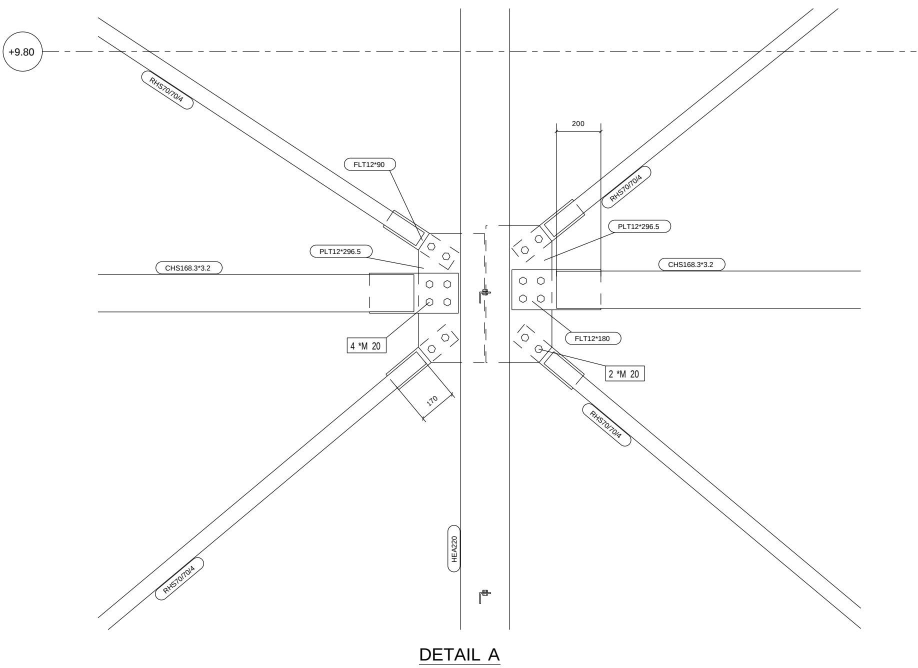
DETAIL A
