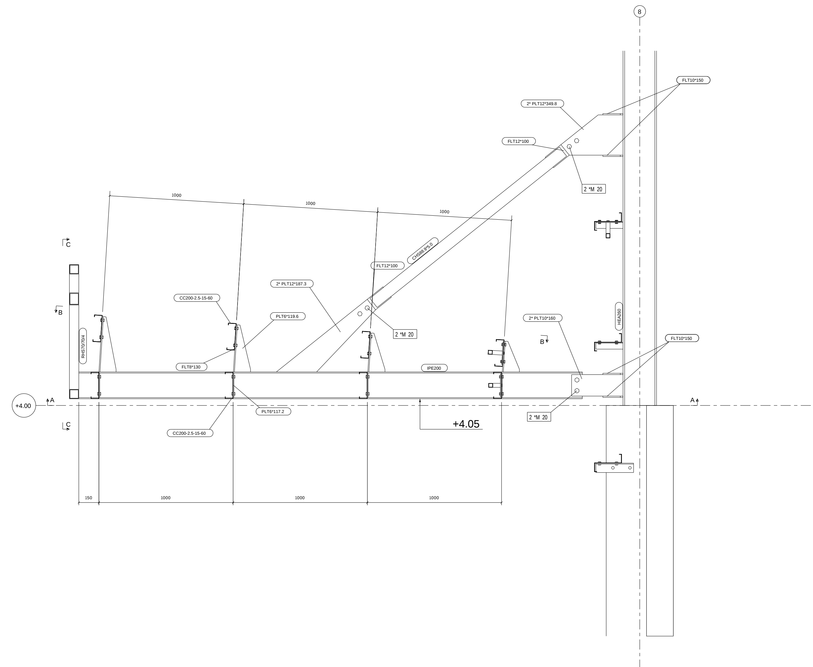
DETAIL A
